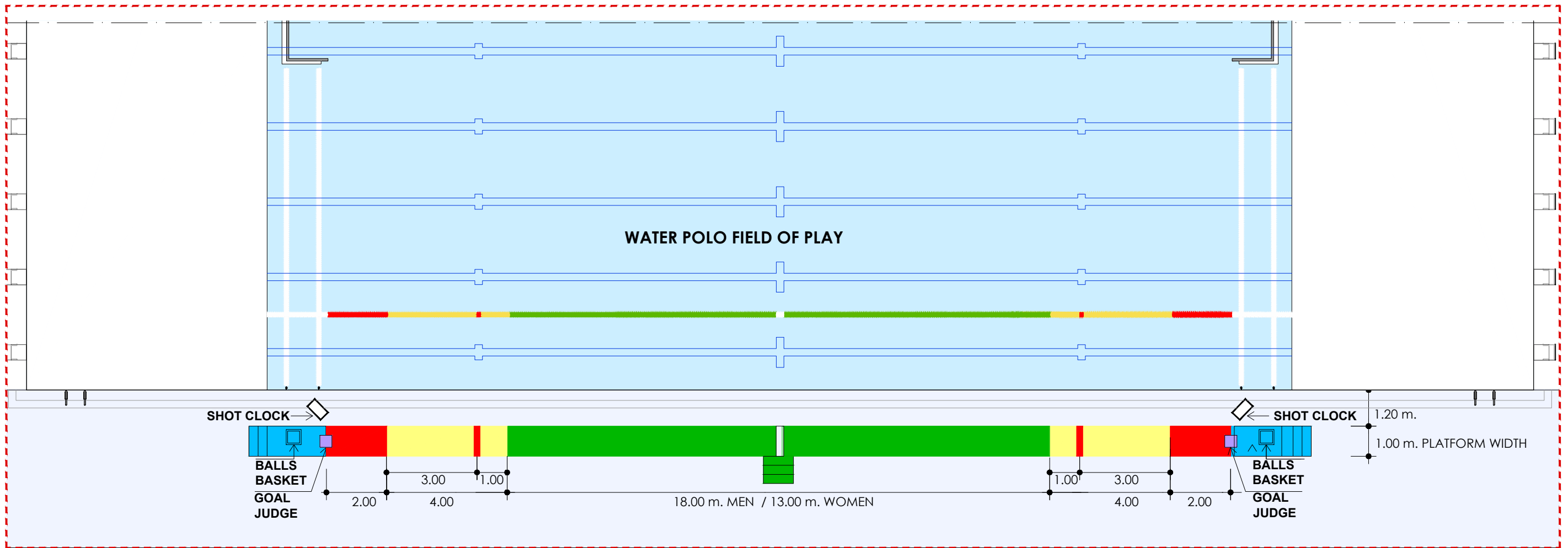
PLAN
