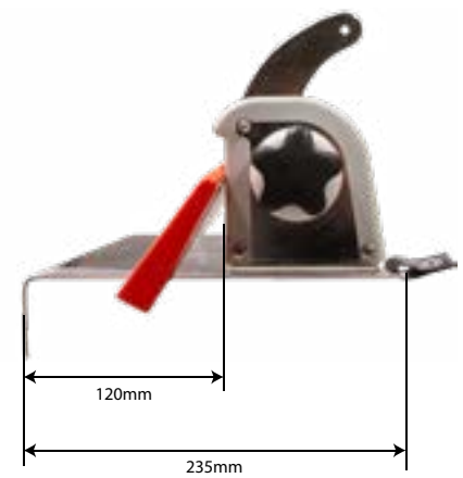
Backstroke Starting Device Long
