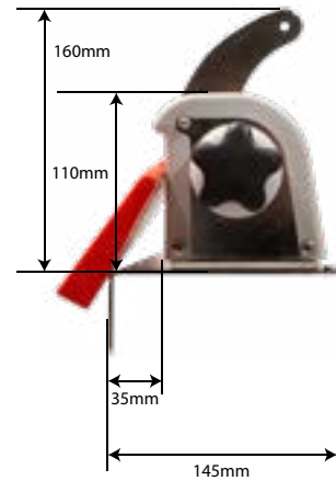
Backstroke Starting Device Long
